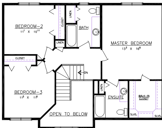
SECOND FLOOR AREA = 839 S.F.
